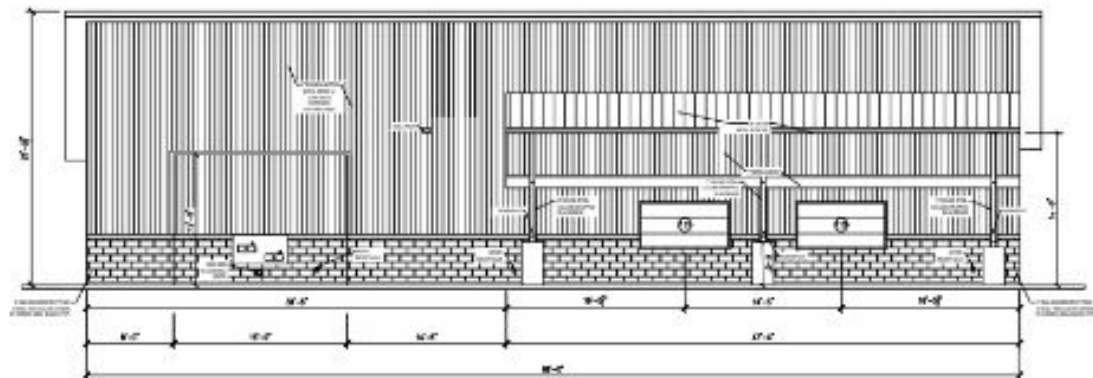
NORTH ELEVATION SCALE: 3/16" = 1'-0"
